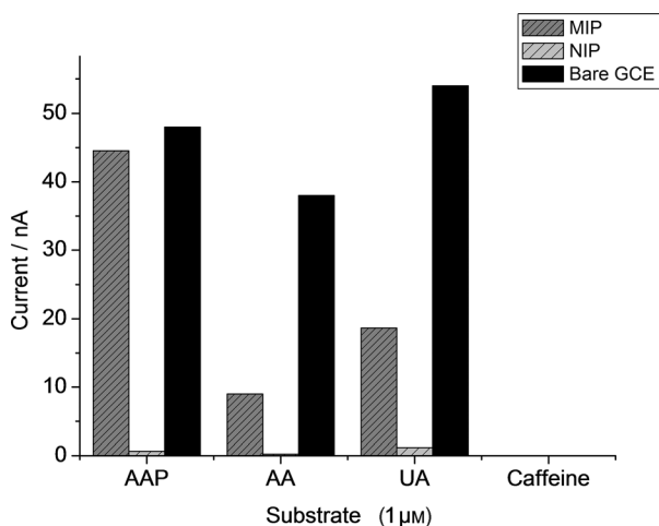
Figure 3. Comparison of the signals of the template and interfering substances on bare, nonimprinted, and AAP-imprinted GCEs.
